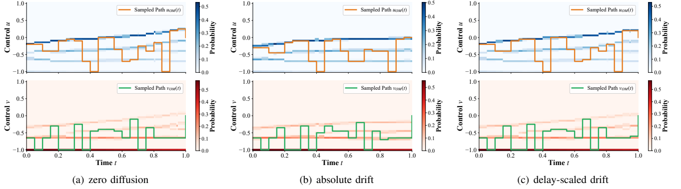
Fig. 2. Mixed strategy distribution under different designs for the diffusion term of \tilde{G} .
